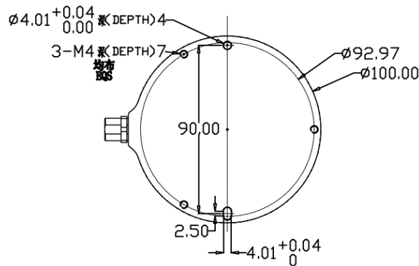
Figure 1.5 CH32R Lidar Base (unit: mm)
