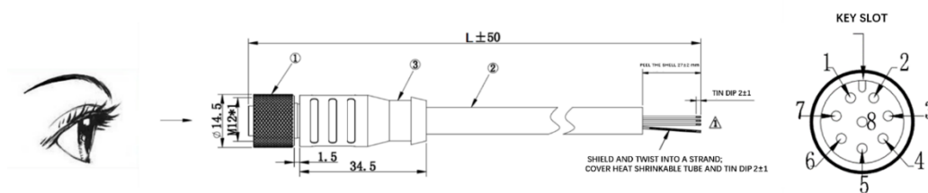
Figure 2.4 CH32R Lidar Extension Cable (unit: mm)
