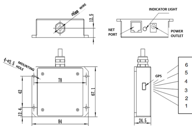
Figure 2.5 Interface Box
