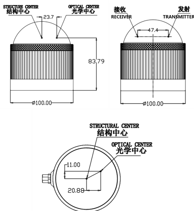
Figure 1.4 CH32R Mechanical Drawing (unit: mm)
