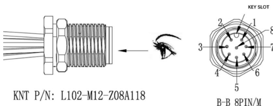
Figure 2.1 Cable Connector on the Lidar Base
