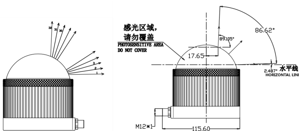
Figure 1.2 Laser Beam Distribution
