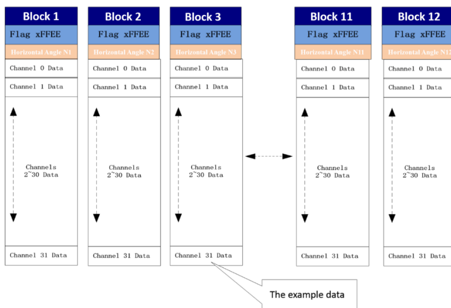
Figure 7.1 Single Echo Data Block Structure
