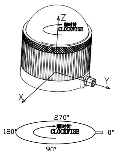
Figure 1.3 Coordinates & Scanning Direction
